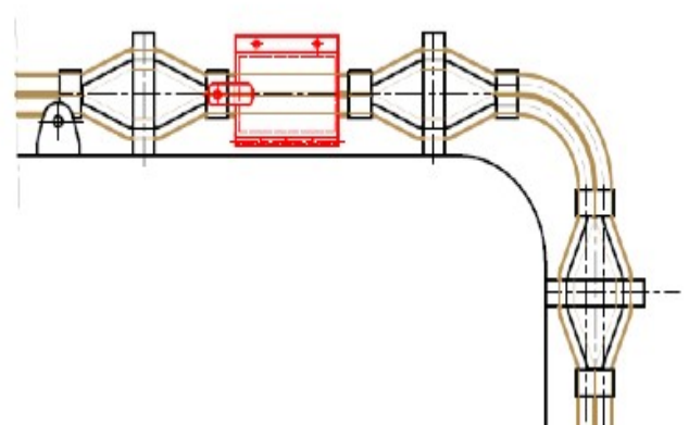
Figure 8c: Design of the securing device
