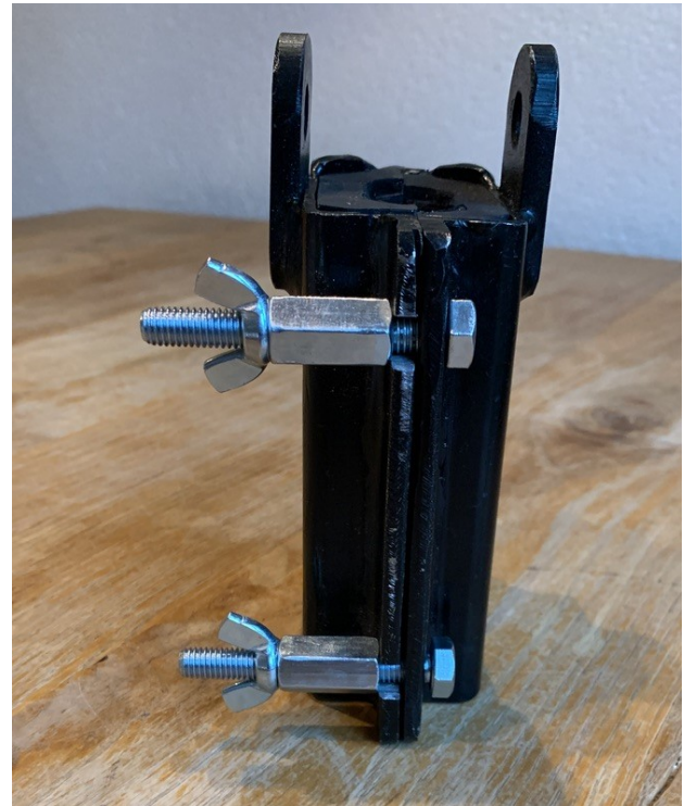
Figure 9c: Securing device with mild steel wingnuts
